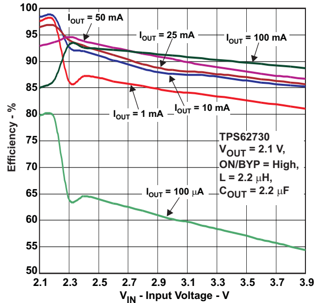
Figure 2. Efficiency vs Input Voltage
